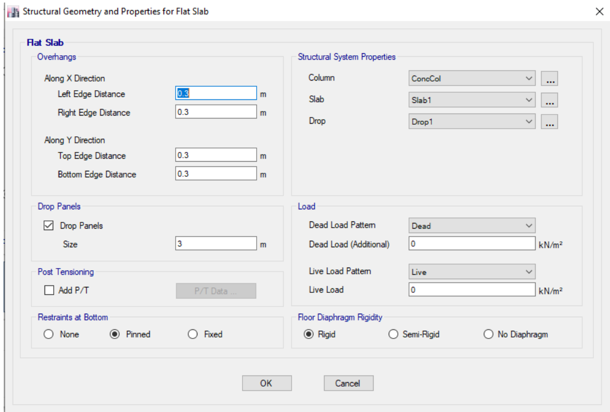
Fig 10 Structural Geometry and Properties for Flat Slab
