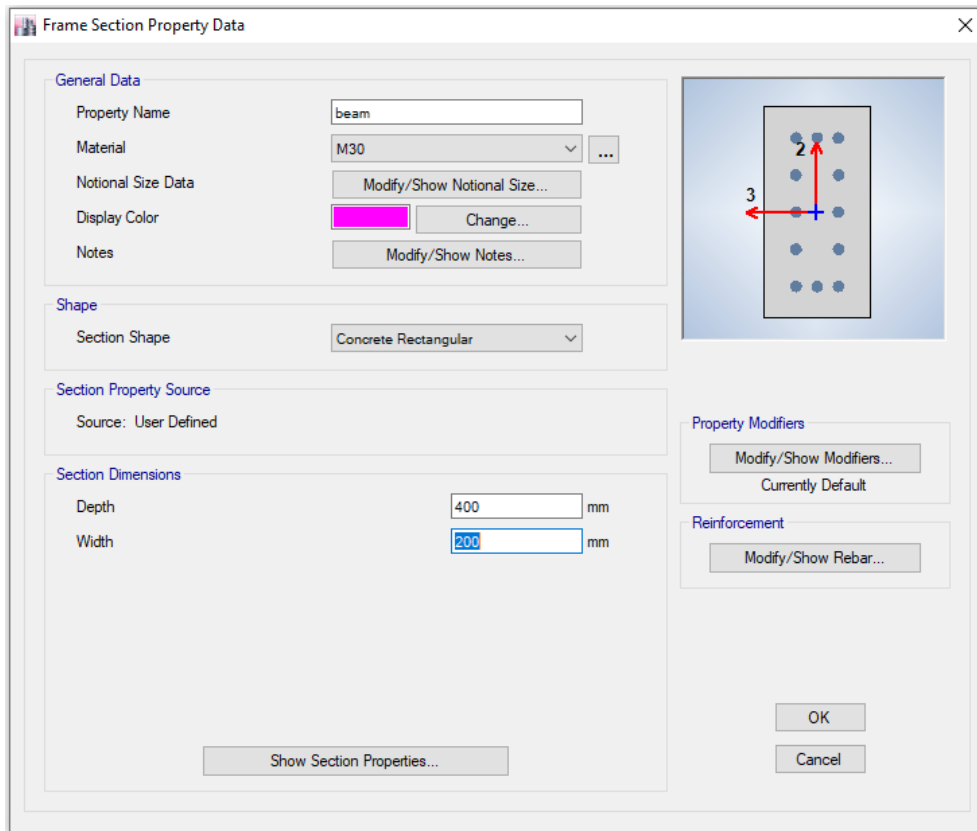
Fig 7 Section Properties for Beam
