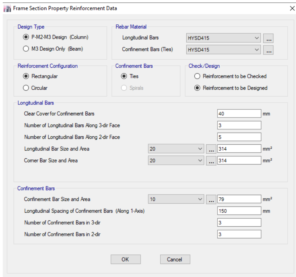
Fig 8 Defining section properties of beam and column.
