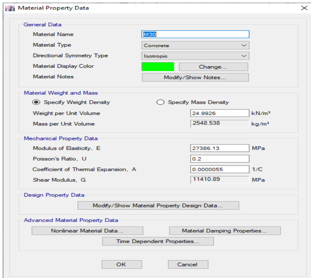
Fig 4 Material Properties for Concrete
